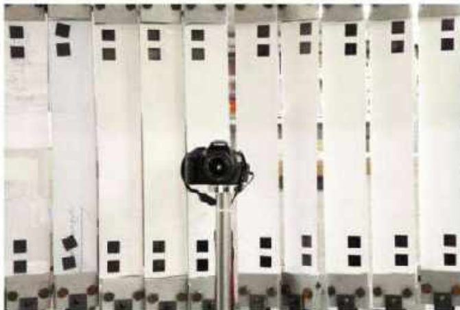
Figure 5.2 Example photo for the optical analysis of the elongation of the strips
