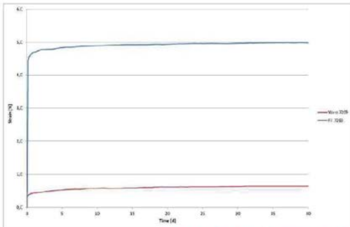
Figure 6.1: Creeping behaviour for the material VALMEX® FR 1000 MEHATOP F - type III 7269 5246 with the loads given in Tab. 5.1
